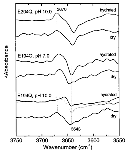
FIGURE 8: O—H stretch region of FTIR difference spectra of hydrated or dry films of E204Q, E194Q, and E194Q/E204Q in 1 M KCl, recorded at 243 K at pH 7.0 and 10.0, as indicated. The dotted line corresponds to the spectrum of a hydrated film of E194Q in 75 mM \text{Na}_2\text{SO}_4 , at 243 K and pH 10.0.
