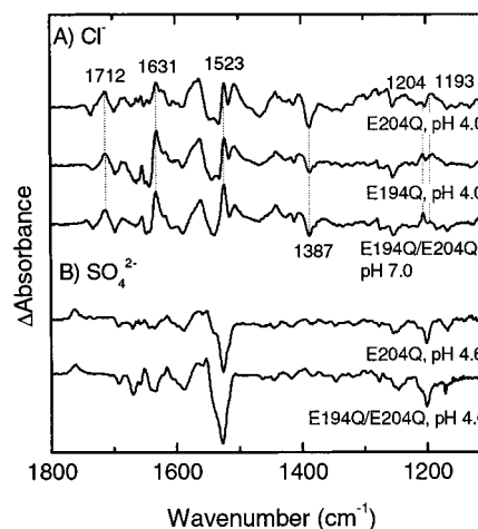
FIGURE 3: FTIR difference spectra recorded at 277 K of (A) hydrated films of E204Q, E194Q, and E194Q/E204Q in 1M \text{KCl} at pH 4.0 and 7.0 and (B) hydrated films of E204Q and E194Q/E204Q in 75 mM \text{Na}_2\text{SO}_4 , at pH 4.6 and 4.0, respectively.
